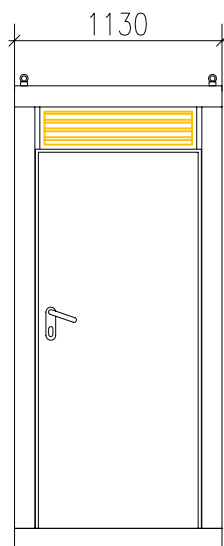
ALZADO PRINCIPAL
