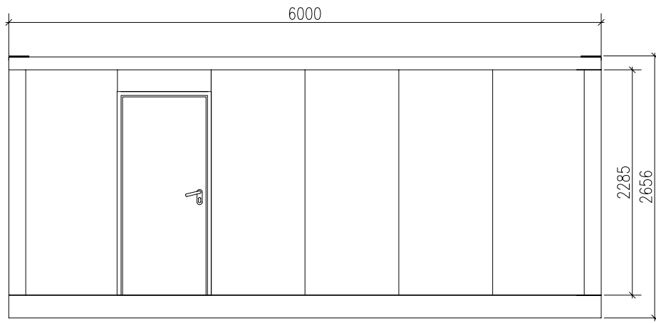
ALZADO PRINCIPAL
