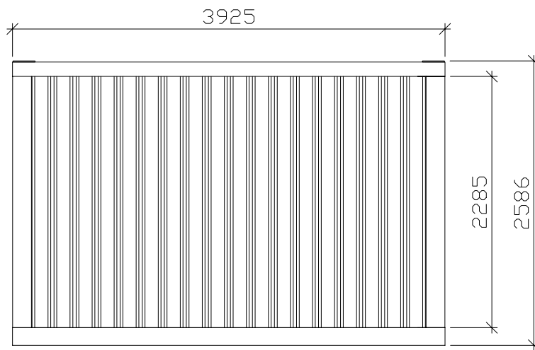
ALZADO PRINCIPAL
