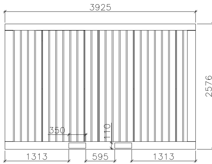
ALZADO PRINCIPAL
